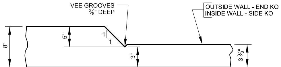
SECTION 1-1
