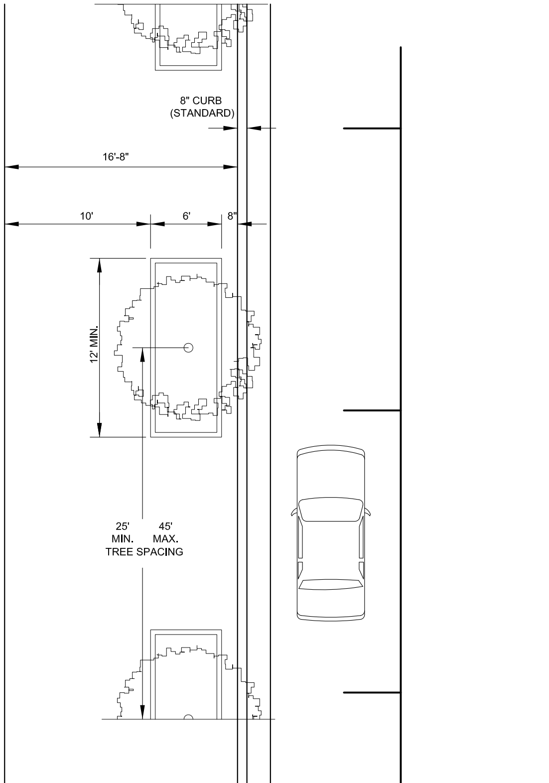
SIXTEEN FOOT EIGHT INCH SIDEWALK AND PLANTING AREA
