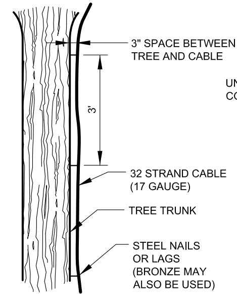
CROSS SECTION 32 STRAND CABLE INSTALLATION
