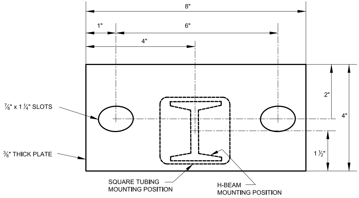
PLATE DETAIL
