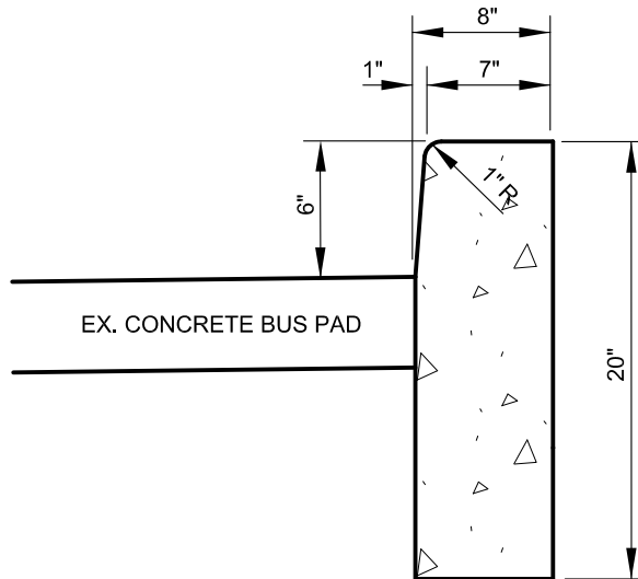
SPECIAL BC TYPE 'A' CURB
