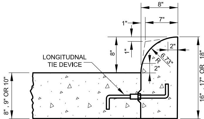
STANDARD TYPE 'A' MODIFIED CURB
