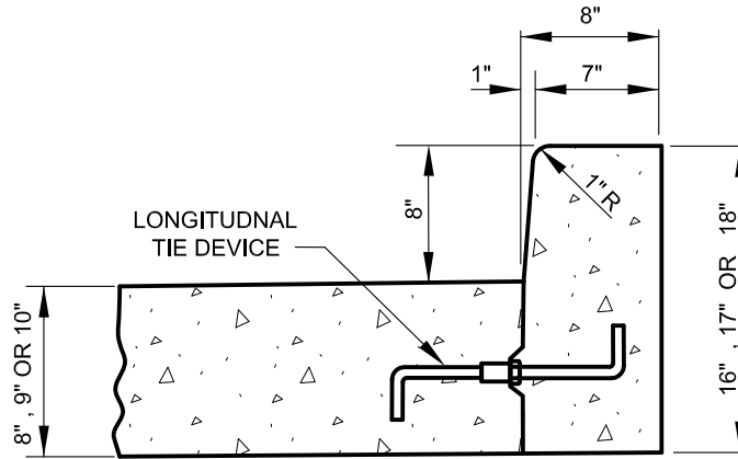
STANDARD TYPE 'A' CURB
